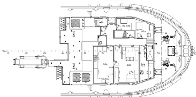
Forecastle deck
