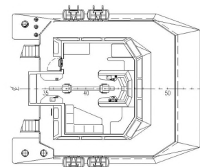
Wheelhouse
