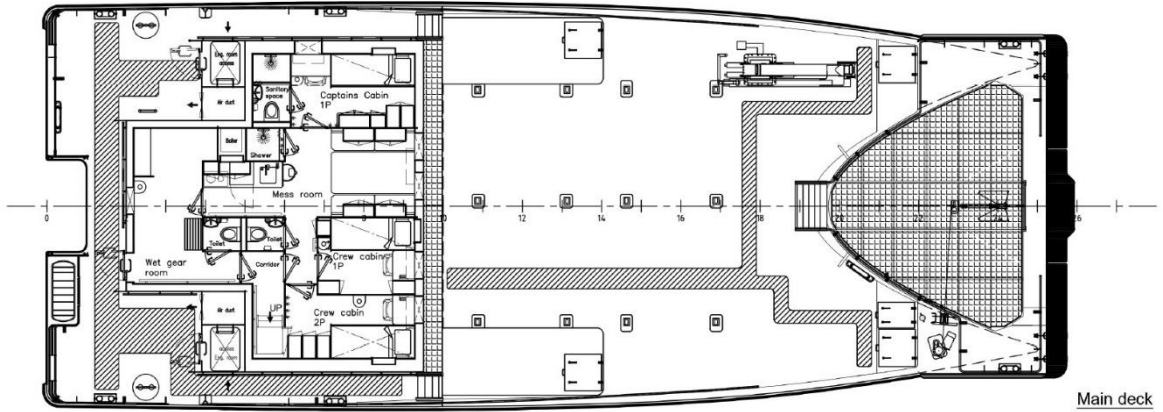
Main deck
