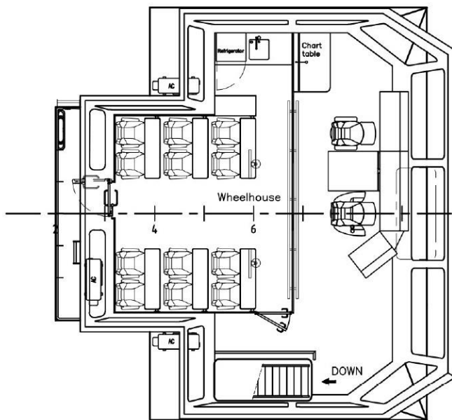
Bridge deck
