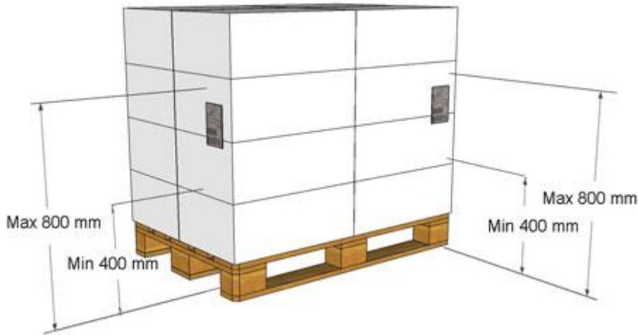
Figure 4; pallet for packaging label
